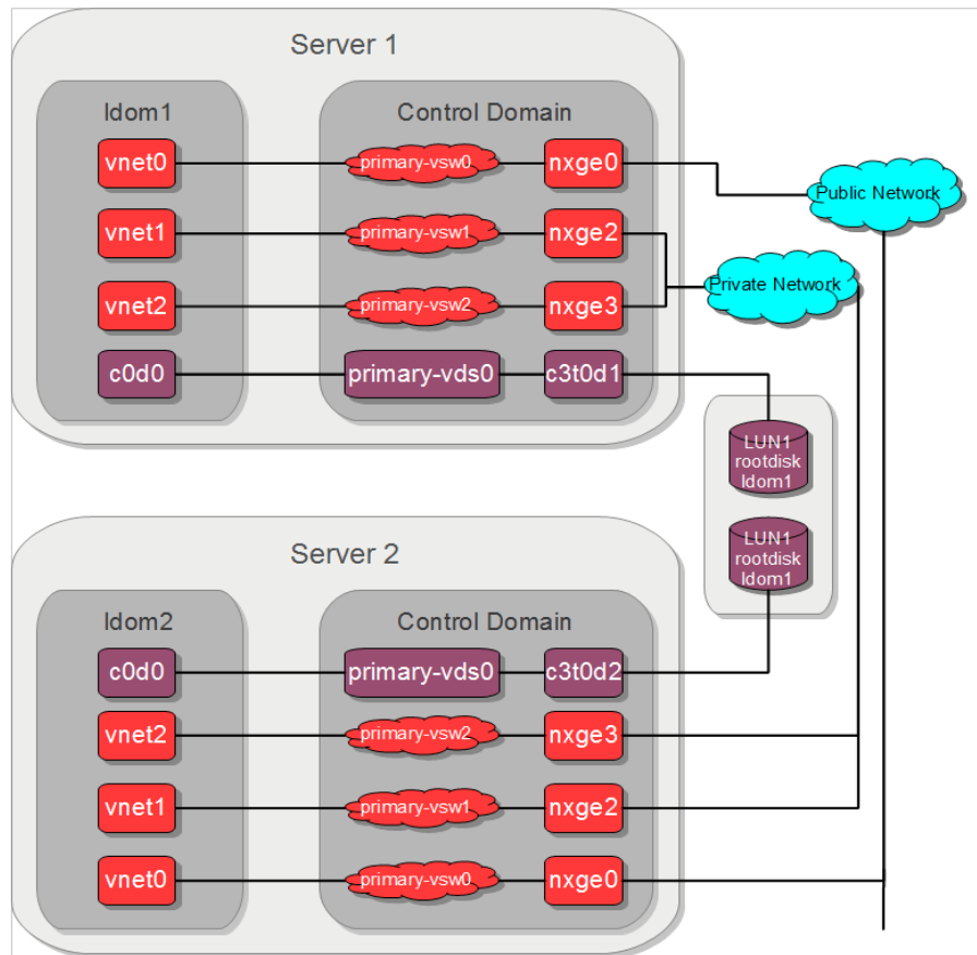
Figure 4: Guest domain initial configuration
