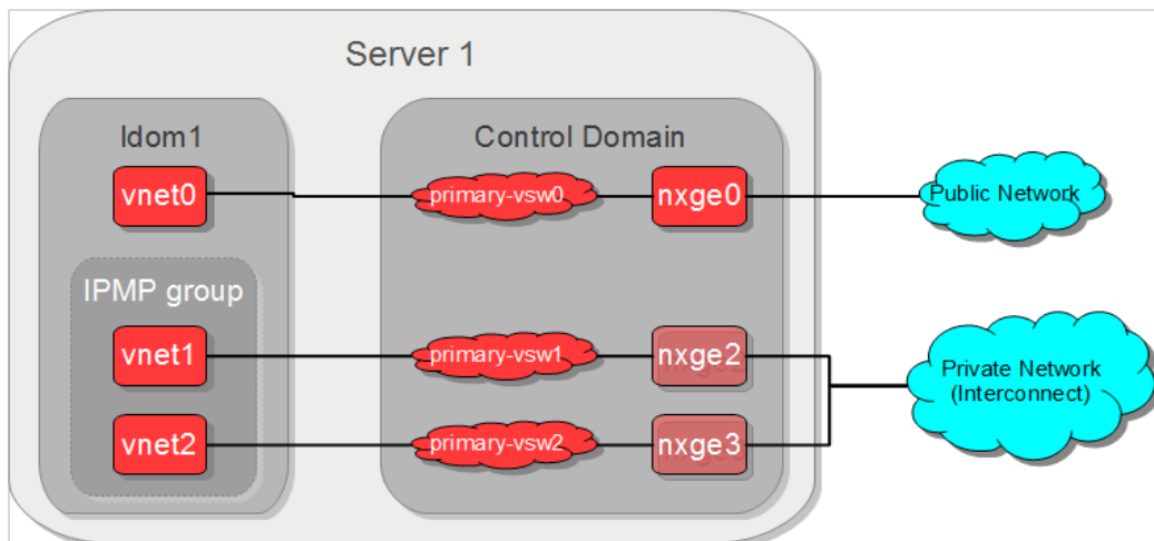
Figure 7: Networking within a physical server
