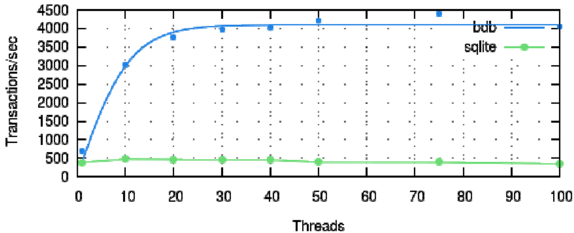
Figure 2 – Workload vs. Concurrent Connections
