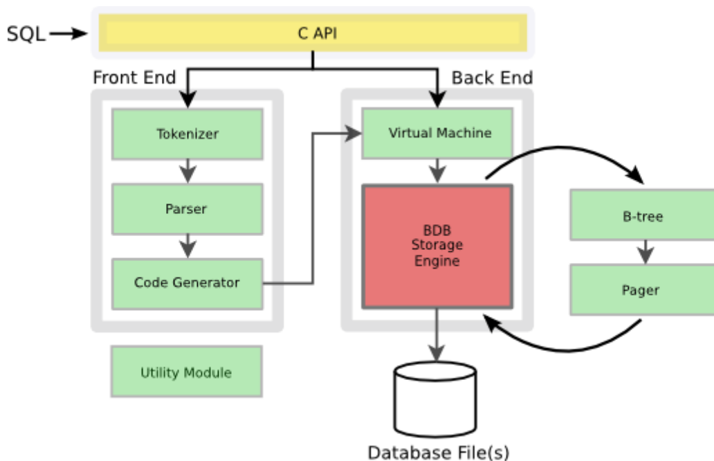
Figure 1 – Oracle Berkeley Database Integration
