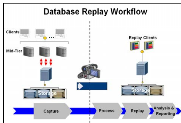
Figure 1: Database Replay Workflow
