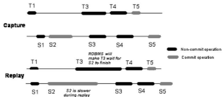
Figure 5: Replay Synchronization Example
