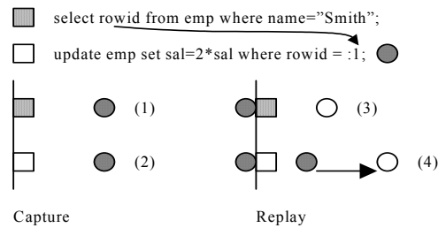
Figure 7: Runtime remapping of system dependent values
