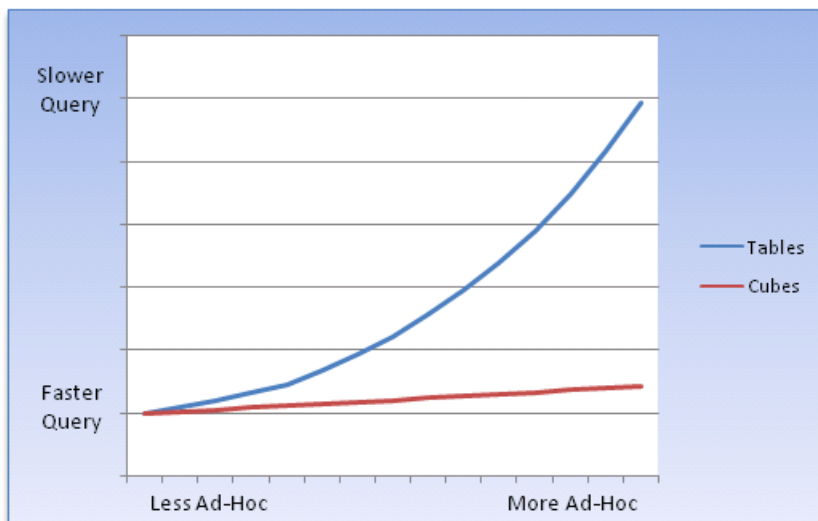
Query performance advantages of cube and cube organized materialized increase as query patterns become more ad-hoc
