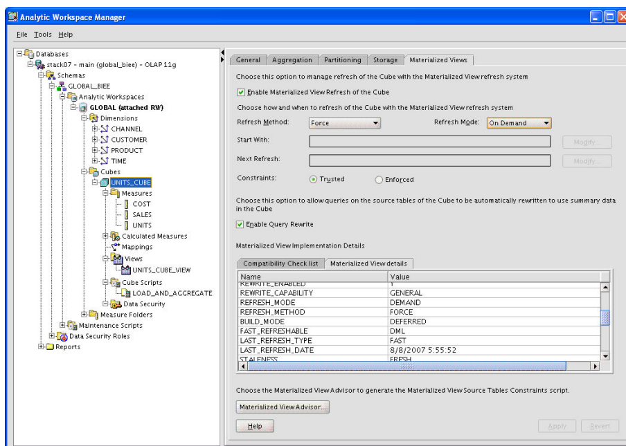
Enabling the cube-organized materialized view for a cube using Analytic Workspace Manager.
