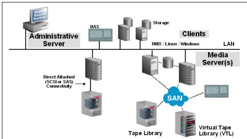
Figure 1: An example of an Oracle Secure Backup domain configuration.
