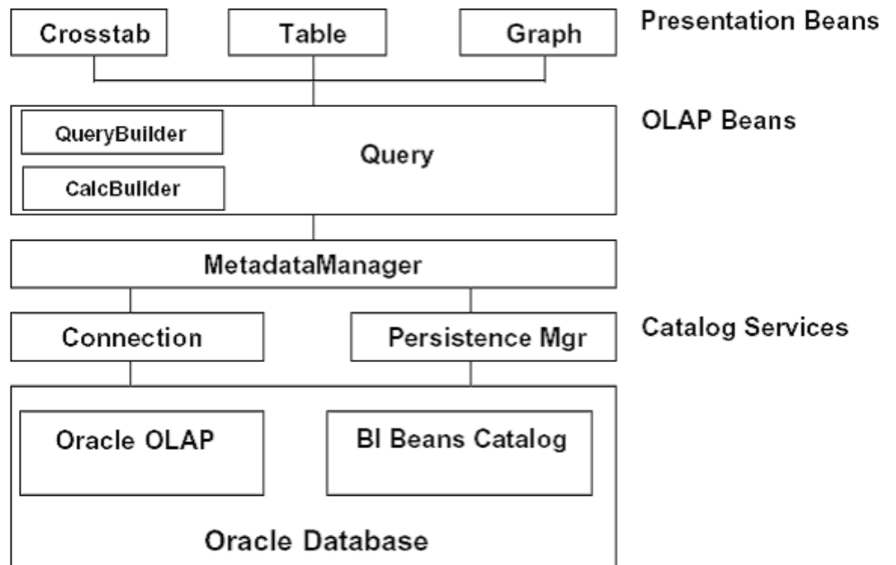
Figure 2: BI Beans Overview
