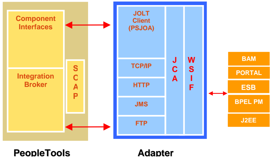
Figure 1: Oracle Adapter for Peoplesoft Architecture Diagram
