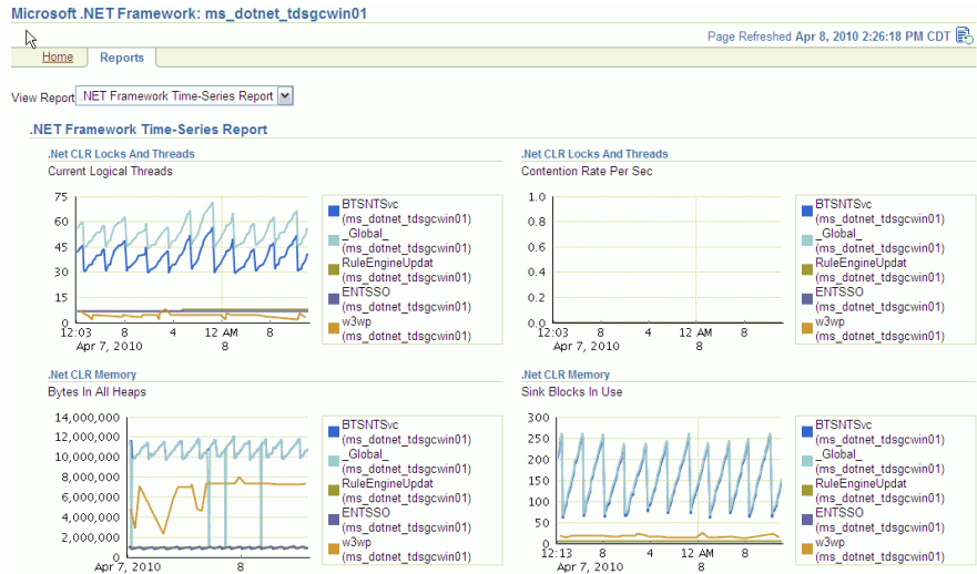
Figure 1. Microsoft .NET Framework Time-Series report.
