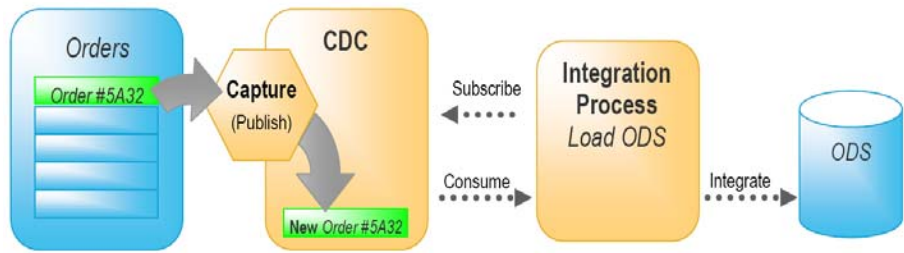
Figure 1: The Changed Data Capture (CDC) framework uses a publish-and-subscribe architecture.
