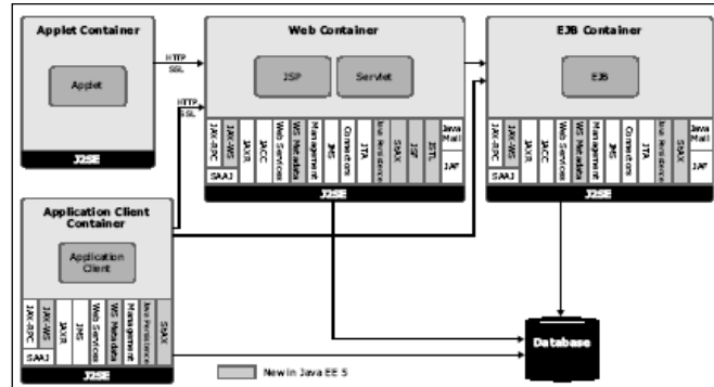
Figure 1: New developer productivity tools in Java EE 5
