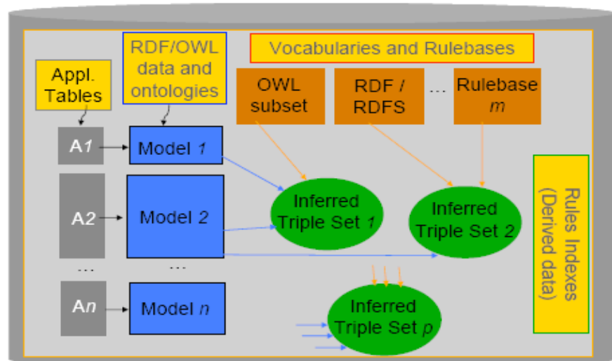
Figure 3. Storage structures in Oracle Database Semantic Data Store
