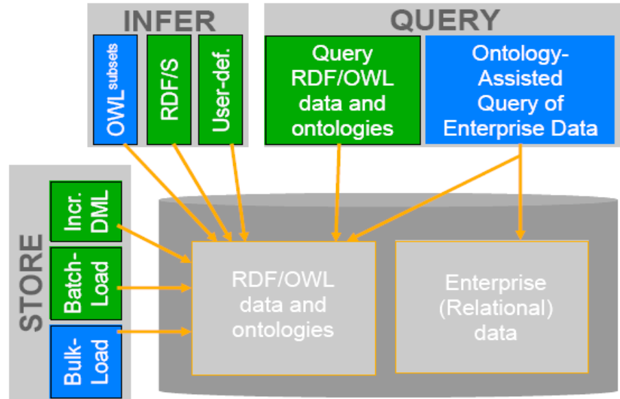
Figure 2. Oracle Database 11g Semantic Data Store
