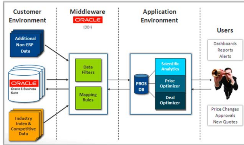
PROS Pricing Solution Suite architecture
