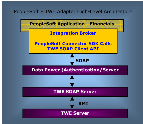
This diagram depicts the integration of ADP's Taxware Enterprise with PeopleSoft Enterprise.
