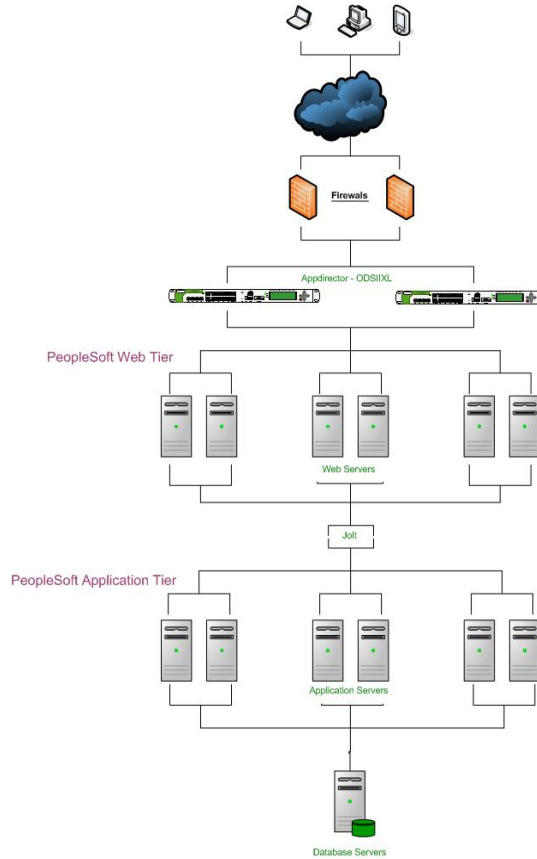
Oracle PeopleSoft Enterprise 9.1 and AppDirector logical topology
