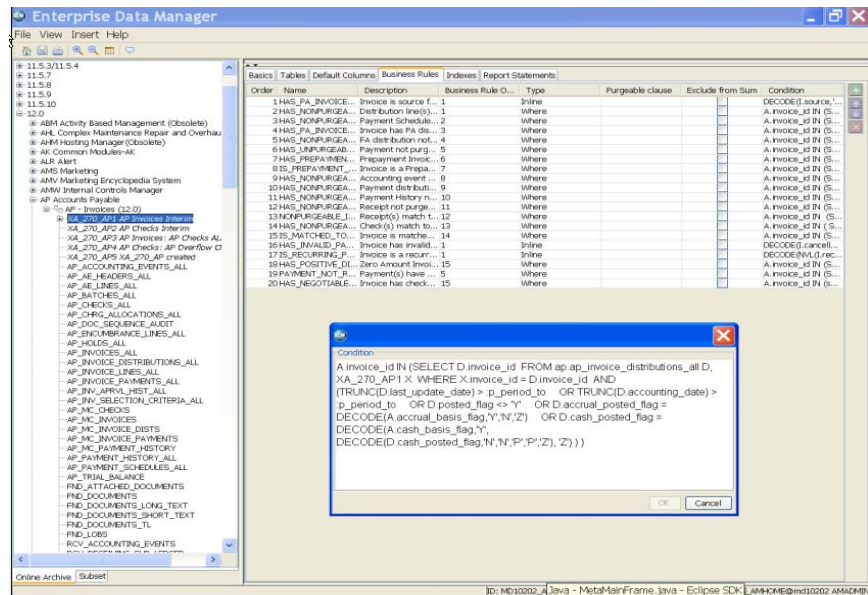
Graphical user interface for customizing archiving templates and business rules.
