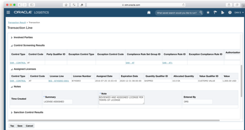
Figure 1. Manually or automatically assign licenses to release holds on transaction lines.
