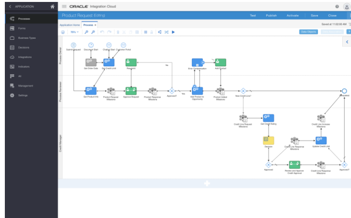
Figure 1: Travel Approval structured (BPMN standards based) process modeling
