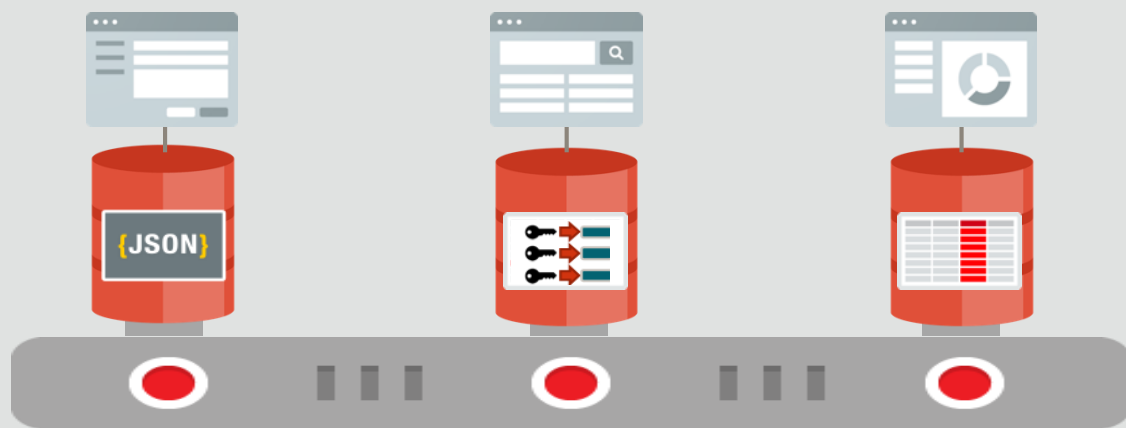
Container Database
