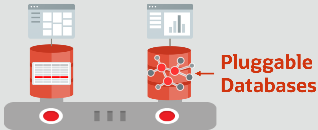
Container Database
