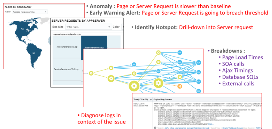
Figure 6. Unified platform. Troubleshoot from APM to LA within the context
