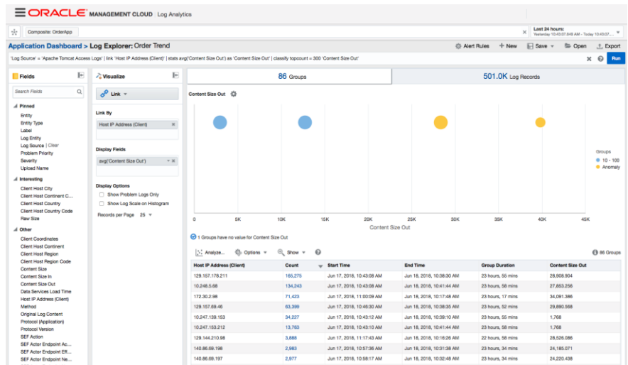
Figure 4. Machine Learning based pattern and anomaly detection
