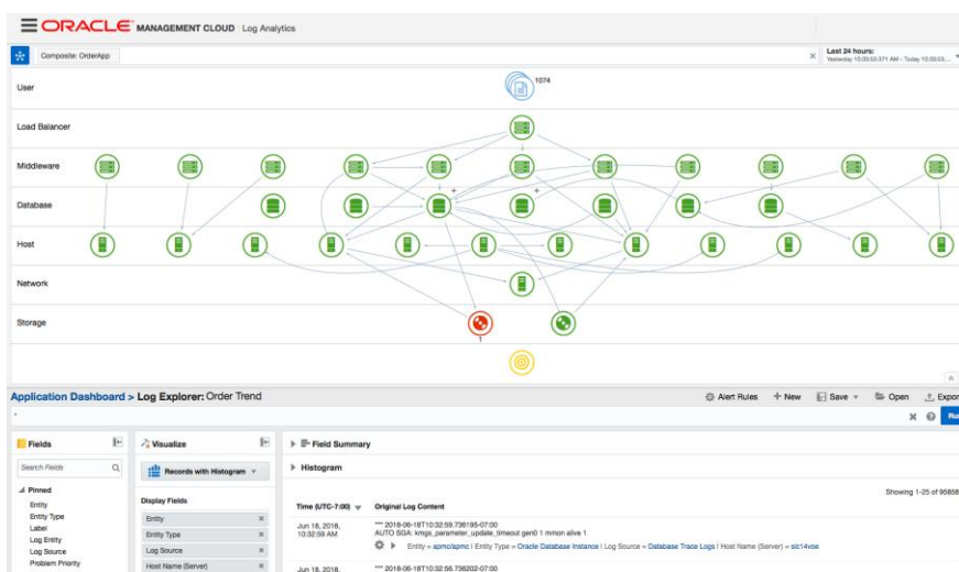
Figure 2. Topology-aware log exploration
