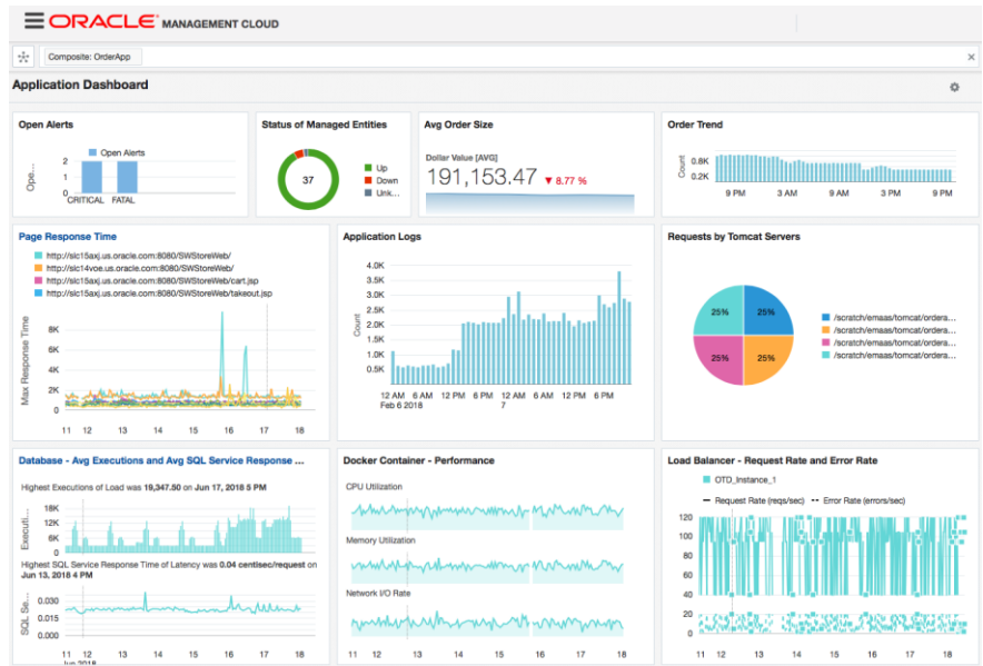
Figure 5. Analyze, build and share compelling dashboards
