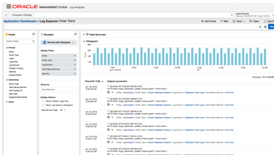
Figure 1. Topology-aware log exploration
