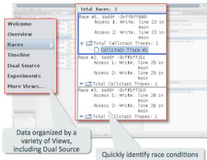
Figure 4. Thread Analyzer GUI Overview
