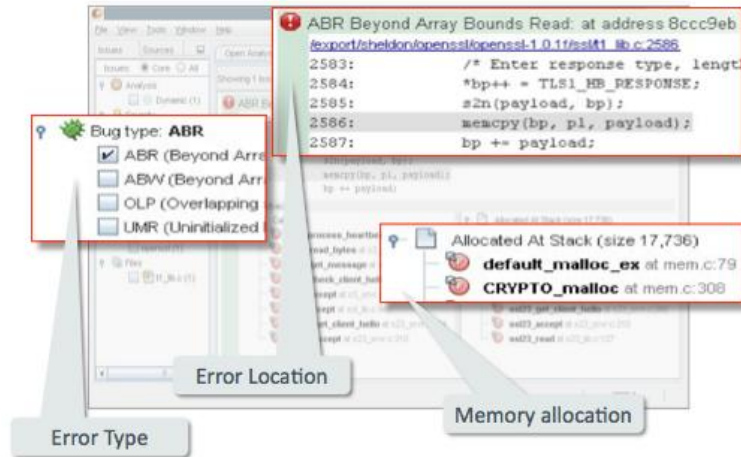
Figure 3. Code Analyzer GUI
