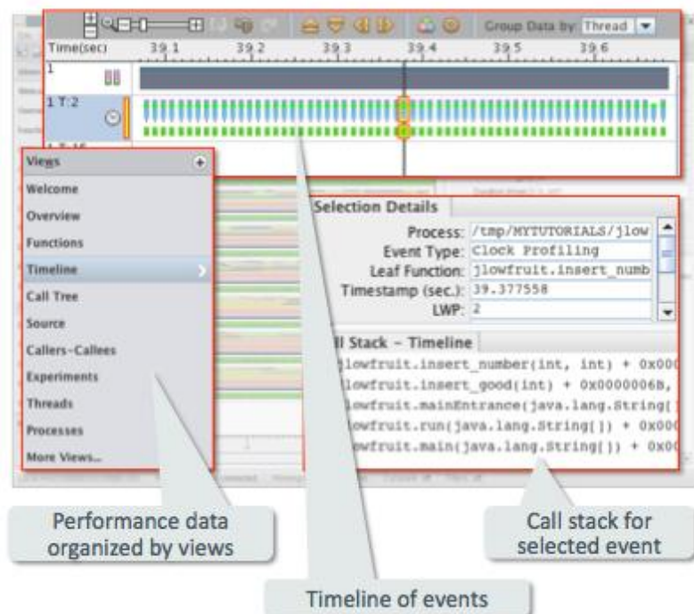
Figure 2. Performance Analyzer Timeline View, demonstrates where time is being spent across multiple threads
