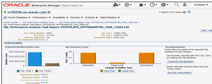
Figure 1. SQL Performance Analyzer Report.
