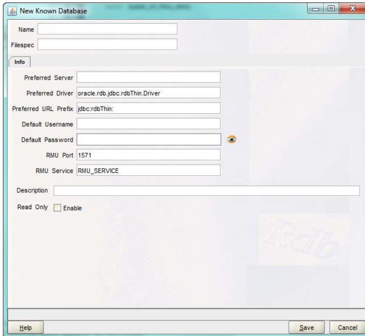
Figure 142 - New Known Database Pane
