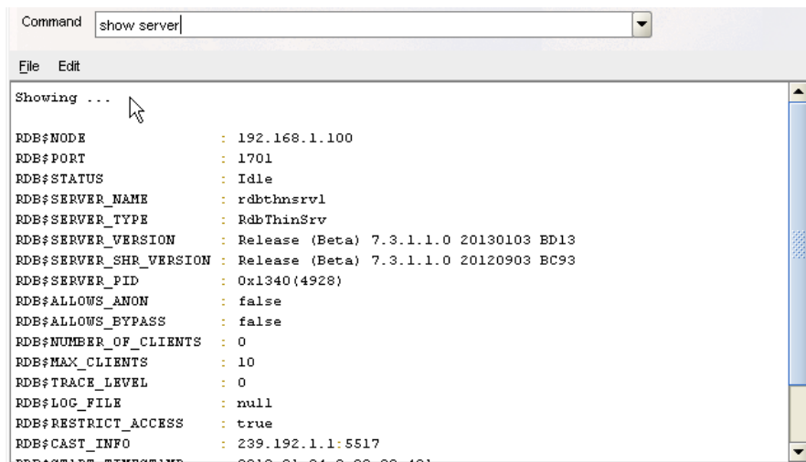
Figure 222 - Results display area
