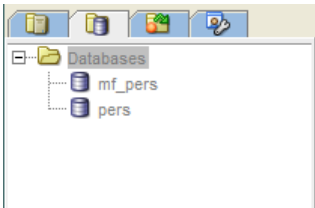
Figure 7 - Database explorer
