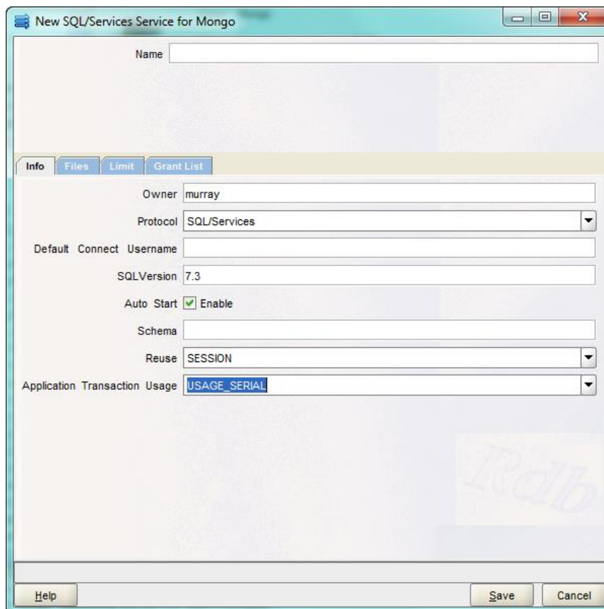
Figure 86 - SQL/Services service Information Pane
