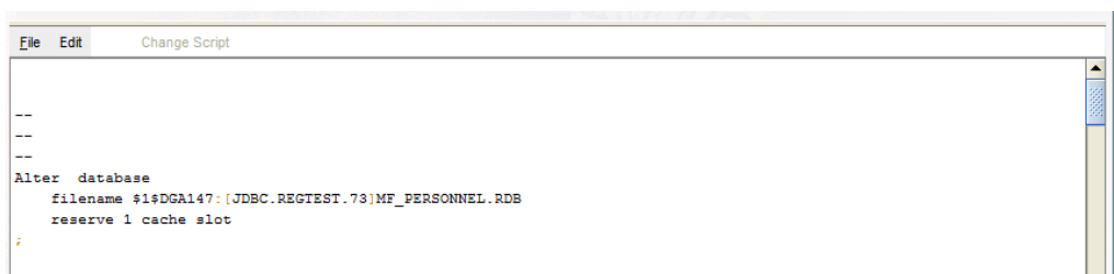
Figure 194 - Suggested SQL syntax in the Change Script buffer
