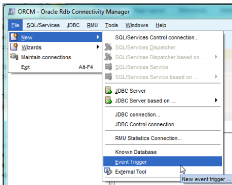
Figure 170 - New Event Trigger menu options
