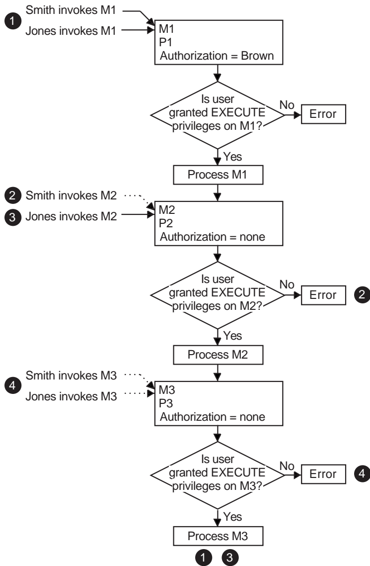
Figure 2–1 Authorization Identifiers and Stored Modules
