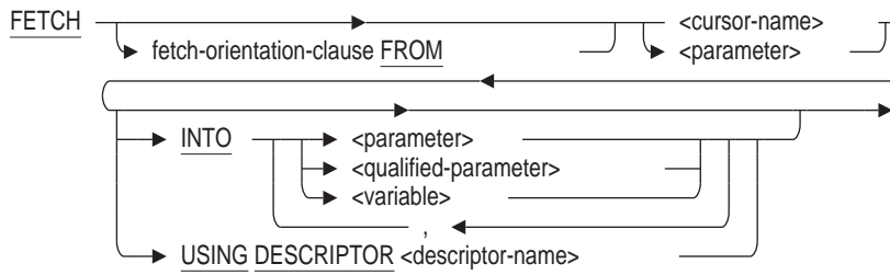
Figure 1–1 Sample Syntax Diagram (FETCH)
