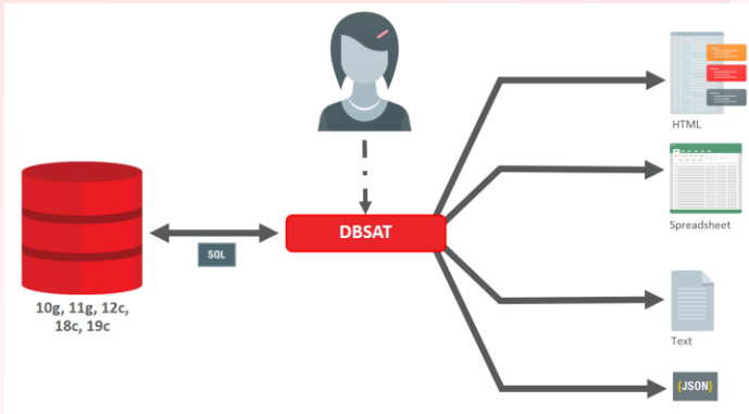
Figure 4. DBSAT Reports.
