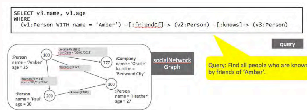
PGQL query
