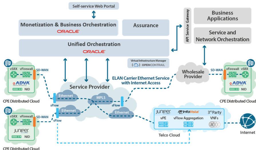
Image 3: End-to-end, standards-based architecture for NaaS orchestration and assurance.
