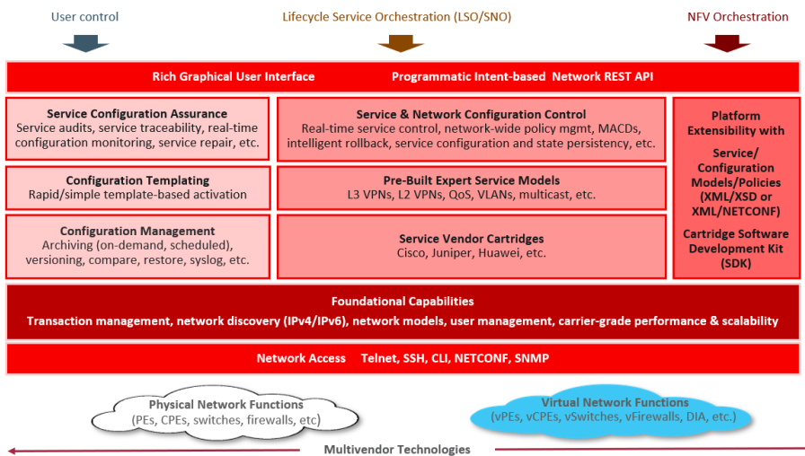
Image 5: IP Service Activator functional architecture
