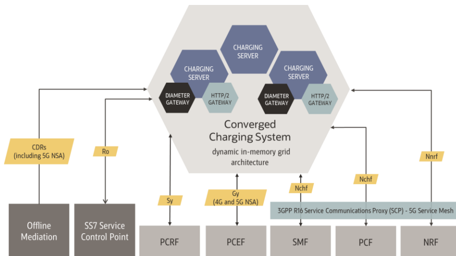
Image 2. Total convergence that supports core network integration with 2G-5G networks
