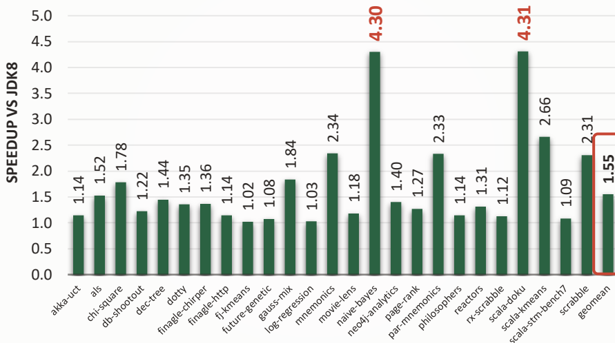
Chart 1: Measured performance of GraalVM Enterprise JIT compiler vs JDK8.
