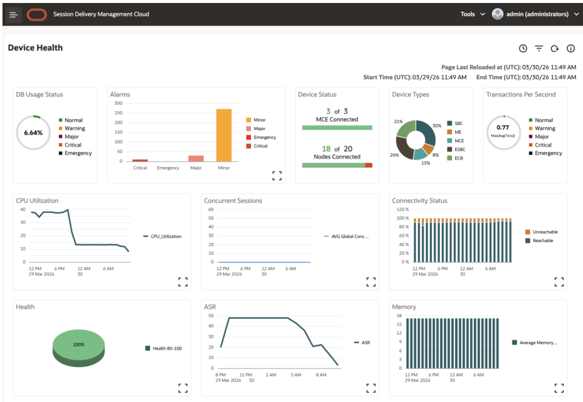
Figure 2. Oracle SDM Cloud dashboard example
