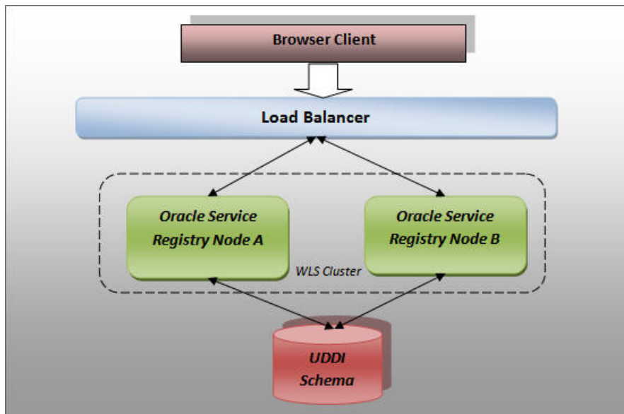
Figure 75. Cluster Architecture
