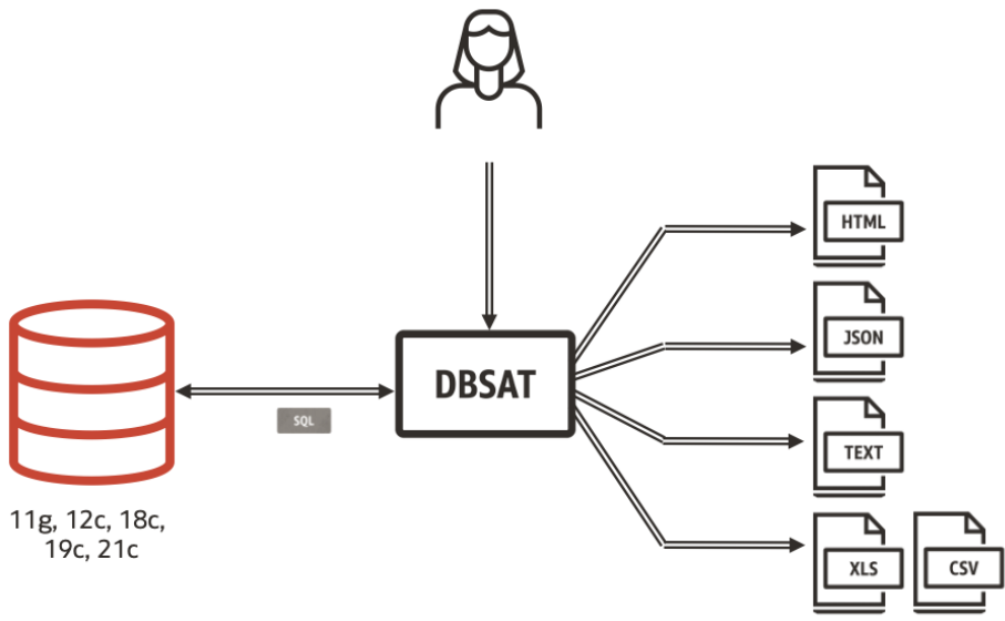
Figure 4. DBSAT targets and output report formats.
