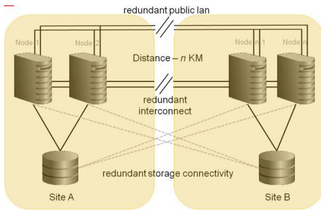
Figure 10: Overall Network Design
