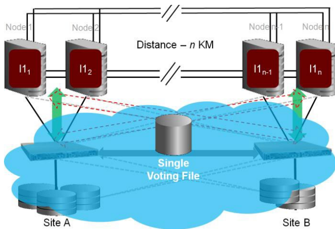
Figure 15: Single Voting File used on Storage Cluster
