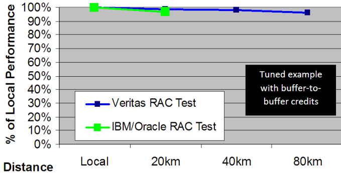
Figure 8: Tuned example – “overall performance impact on applications due to distance”
