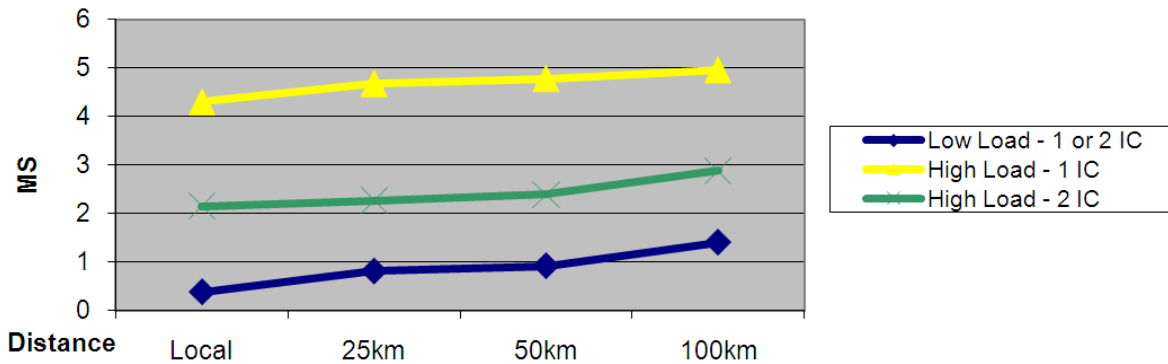
Figure 7: Interconnect Unit Traffic Test Results
