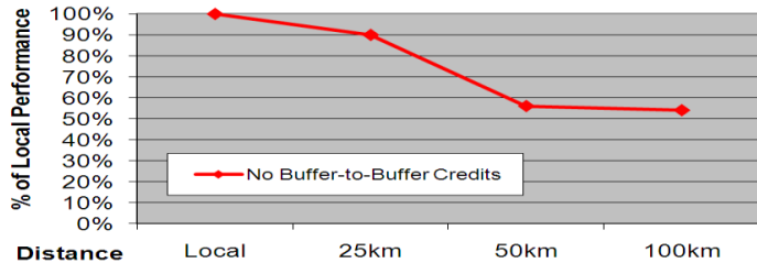
Figure 9: Untuned example – “overall performance impact on applications due to distance”
