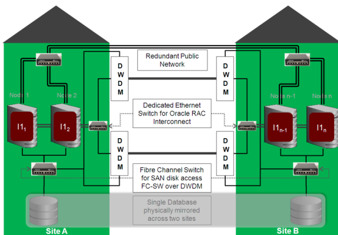
Figure 5: Oracle RAC on Extended Distance Cluster Architecture Overview
