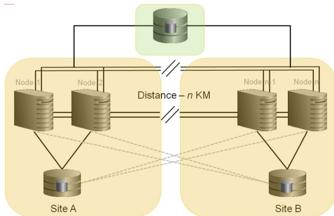
Figure 14: Extended Distance Cluster with Quorum File / Voting File in Third Location
