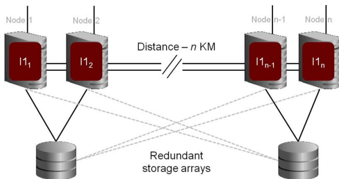
Figure 1: Oracle RAC on Extended Distance Clusters Characteristics
