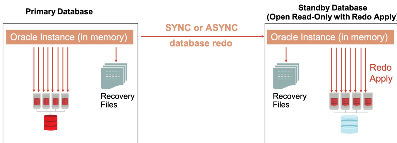
Figure 2: (Active)Data Guard Architecture
