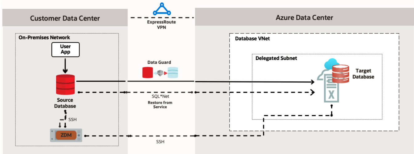
Figure 2. This is a High-Level Architectural overview showcasing the customer data center where the source database and ZDM's server reside. It also shows all connectivity to the target Oracle Exadata Database Service on Dedicated Infrastructure (ExaDB-D) on Oracle Database@Azure.
