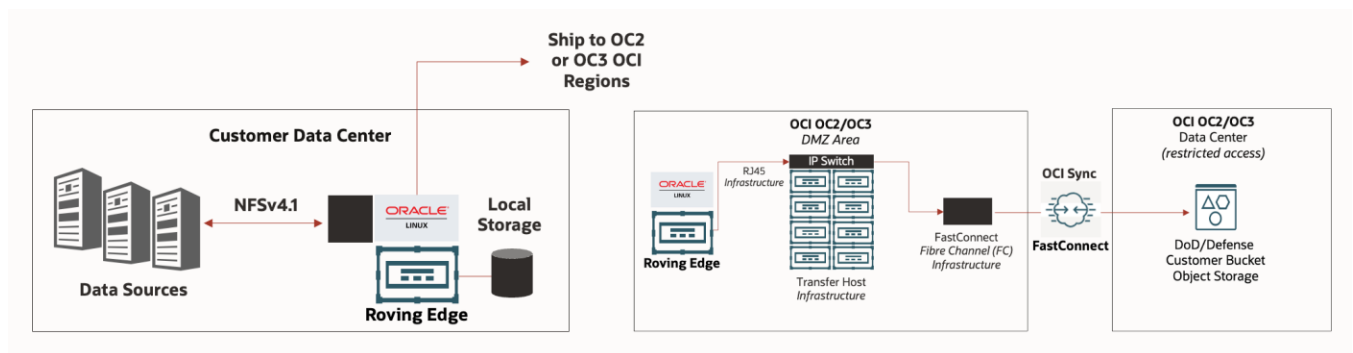
Figure 3. End-to-end architecture diagram of the Roving Edge as Data Transfer Gateway for DoD/Defense customers.
