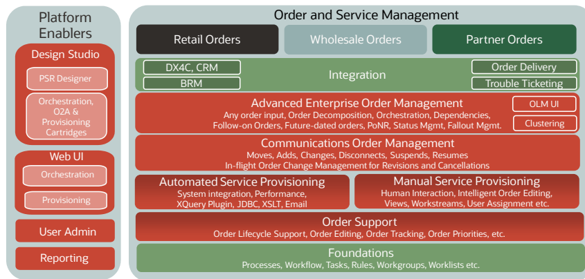
Image Caption 3. Order and Service Management Functional Capabilities
