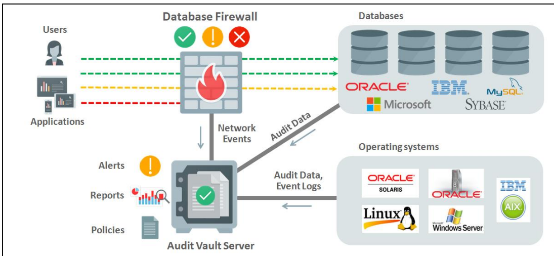
Figure 7: Oracle Database Security Monitoring Controls
