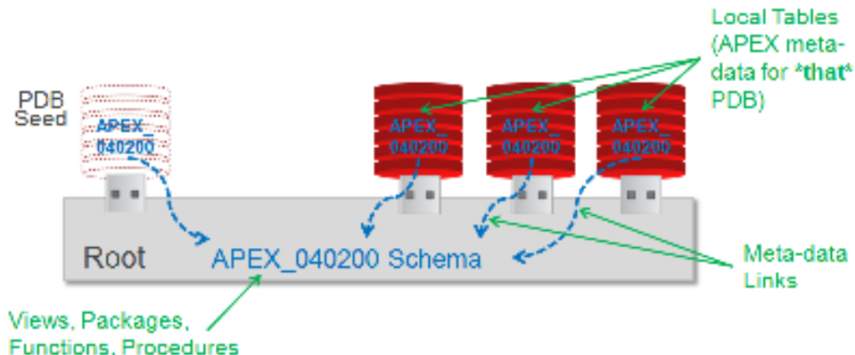
Figure 2 - Default Application Express Installation
