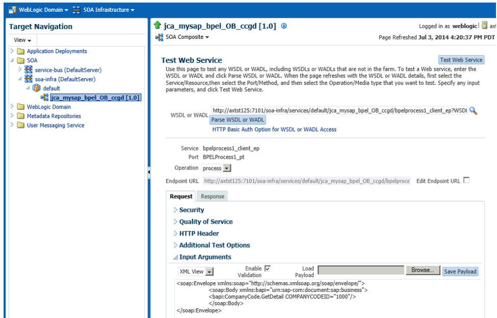
Figure 2–24 Input XML in XML View
