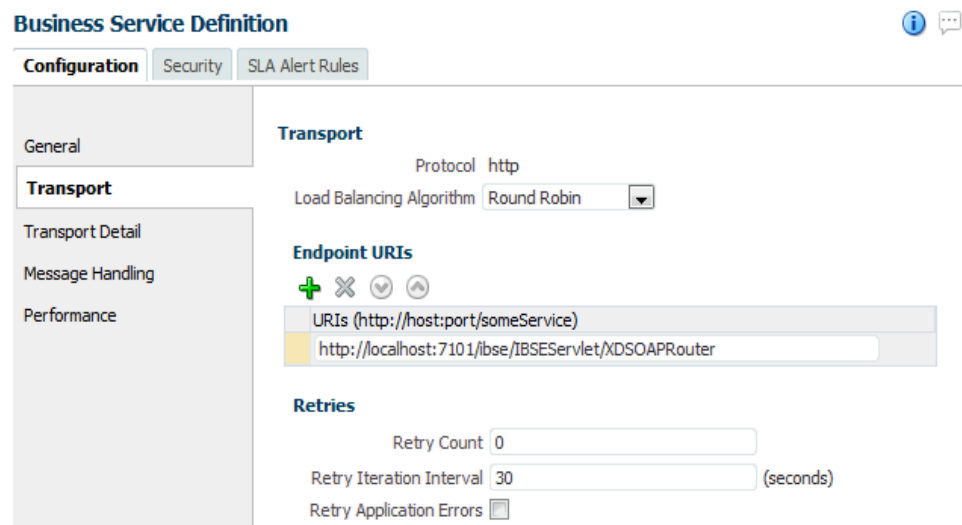
Figure 2–15 Transport Configuration Tab
