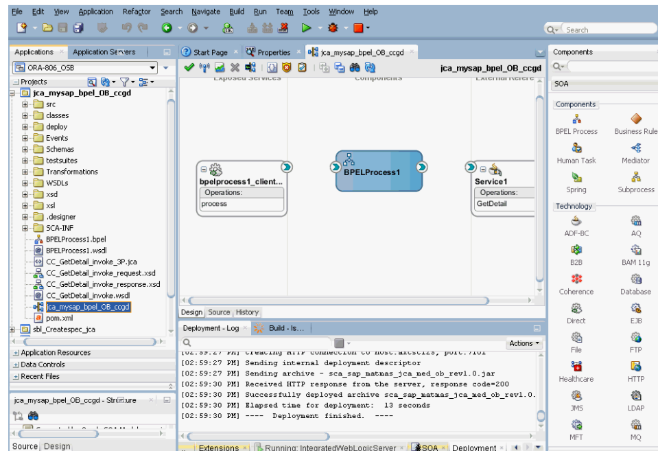
Figure 2–19 Migrated Sample Project
