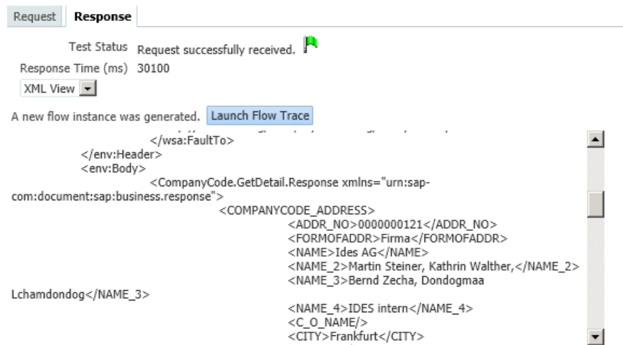
Figure 2–25 Received Output XML
