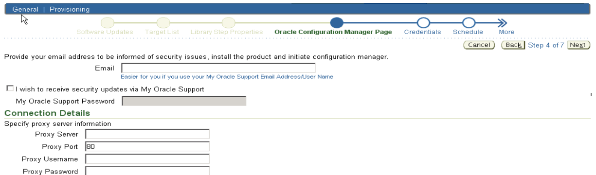
Figure 16: OCM Configuration page
