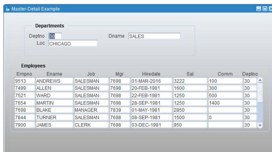
Figure 7: Gradient colored content canvas.
