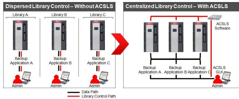
Figure 1. This contrasts the configuration before and after StorageTek ACSLS Manager software is utilized to centralize the control path
